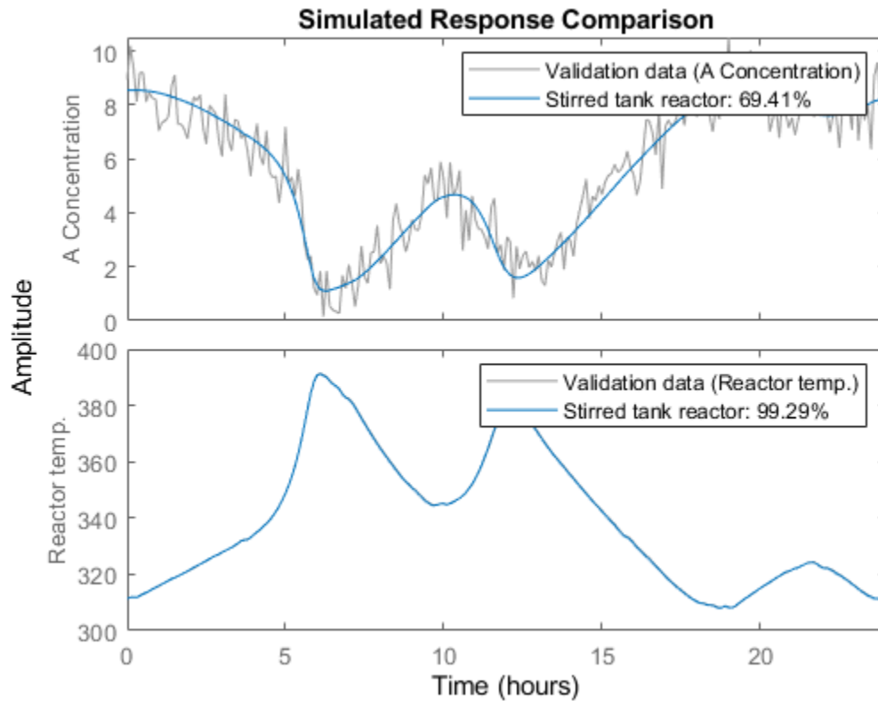
Figure 5: Comparison between the true outputs and the simulated outputs of the estimated CSTR model.
